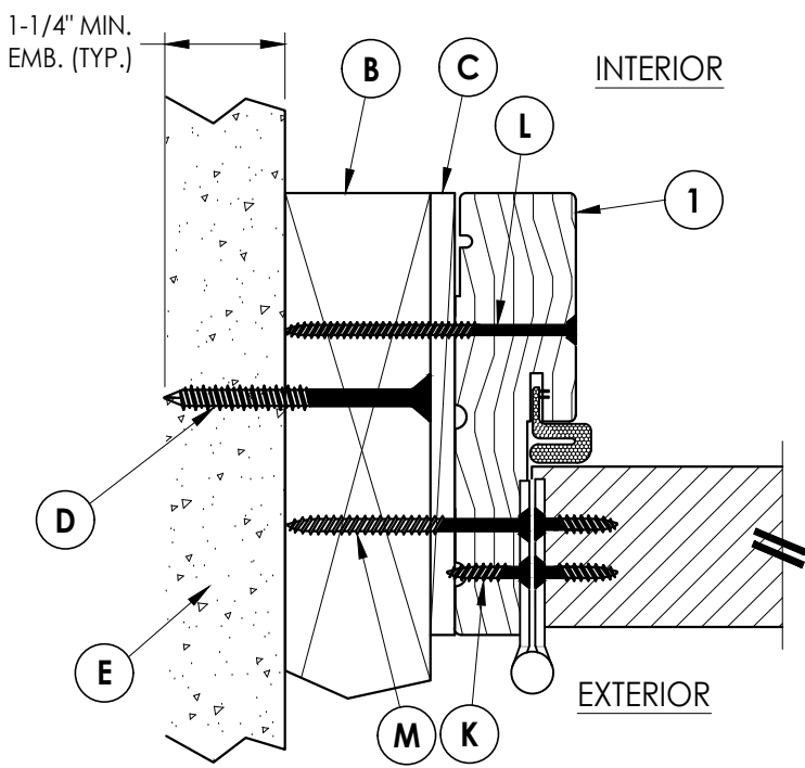
1 HORIZONTAL CROSS SECTION 2 Outswing 2X Buck Construction
