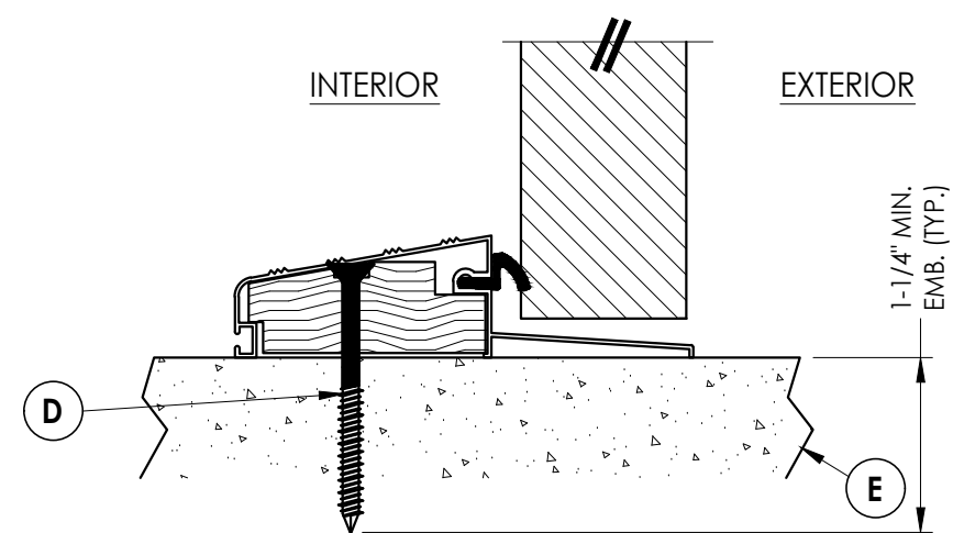
3 VERTICAL CROSS SECTION
