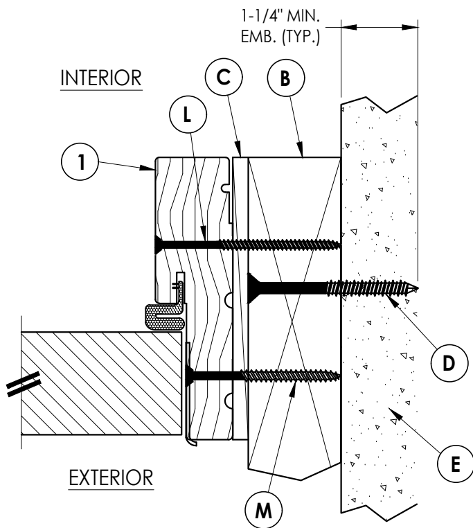
4 HORIZONTAL CROSS SECTION 2 Outswing 2X Buck Construction
