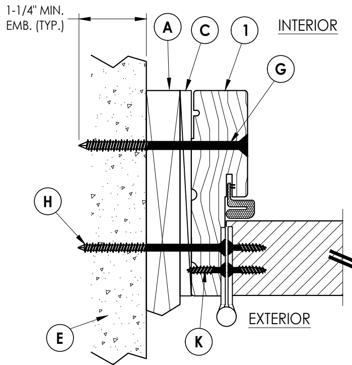
2 HORIZONTAL CROSS SECTION 2 Outswing 1X Buck Construction
