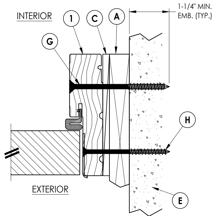
3 HORIZONTAL CROSS SECTION 2 Outswing 1X Buck Construction
